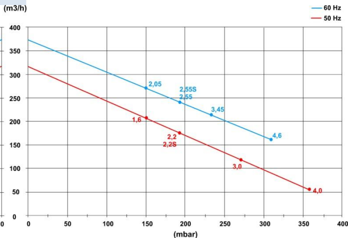
Caudal aspirado / Suction air flow
